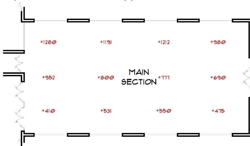
Figure 3: National Library Kaduna reading area's measured illuminations. Source: Field study (2025)
