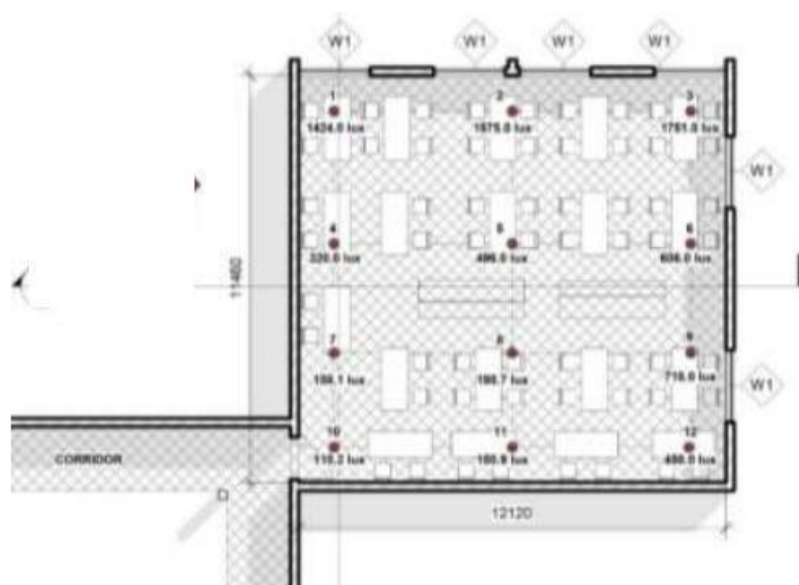
Figure 1: Kaduna State University's conventional reading area's measured illuminations in Kaduna.
