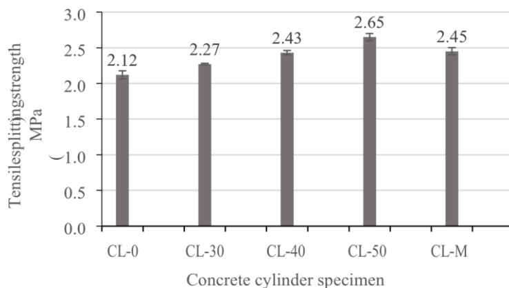
Figure 7. Tensile splitting strength of RTSF concrete specimens
