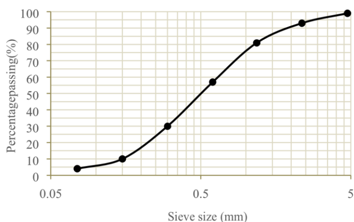
Figure 3. Particle size distribution curve for fine aggregate
