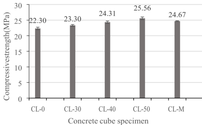
Figure 5. Compressive strength of RTSF concrete specimens
