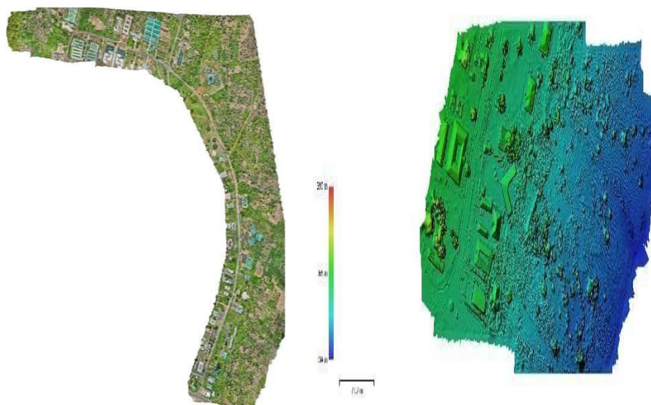
Figure 2a: Orthomosaic Image of the study area Figure 2b: Image of the Dense Point Cloud 3.2
