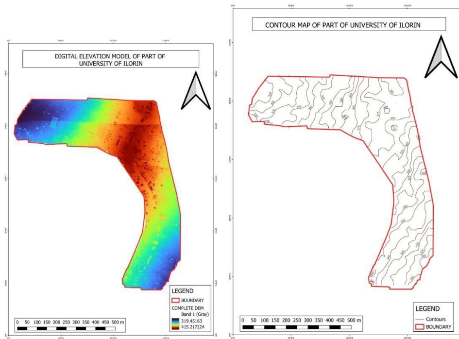
Figure 3a: Digital Elevation Model of the study area Figure 3b: Contour Map of the study area
